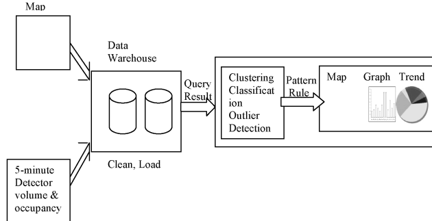
Figure 5 Data-flow and main modules in our system
