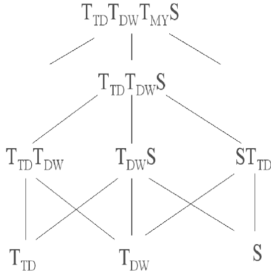
Figure 3 Dimension hierarchy of CubeView
