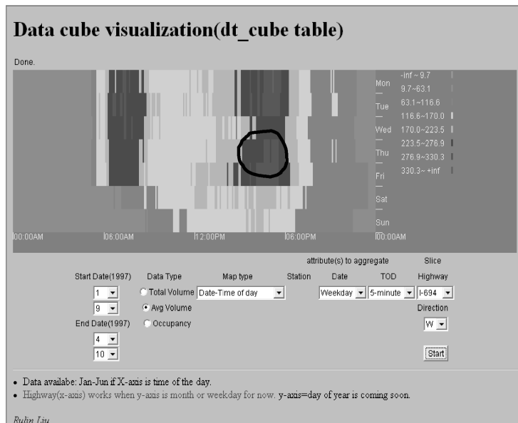
Figure 8 2D representation of time and traffic volume. (Dimension: T_{TD} T_{DW} )
