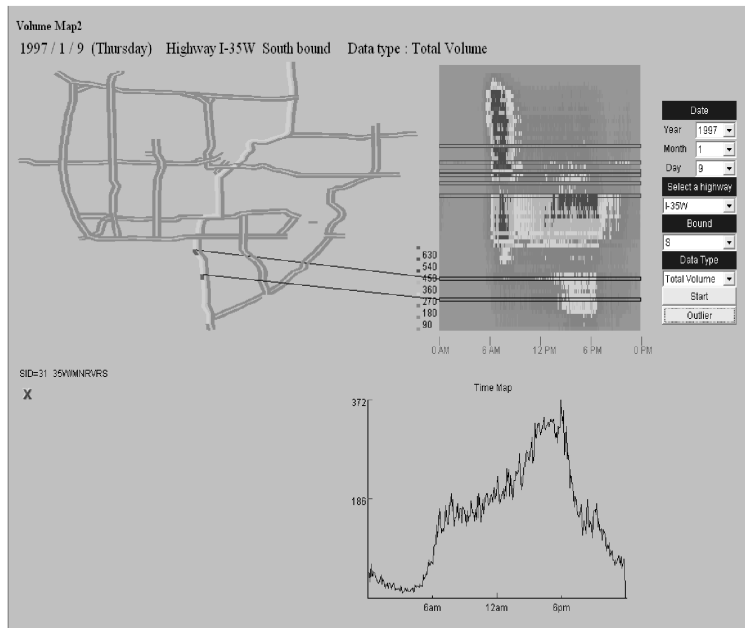
Figure 6 View showing the outliers and traffic patterns for each station on a highway. (Dimension ST_{TD} )
